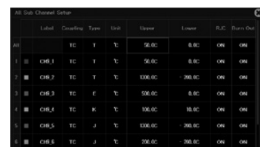
Channel setting screen (DL950)
