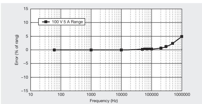
Example of Frequency characteristic under PF = 0 condition
