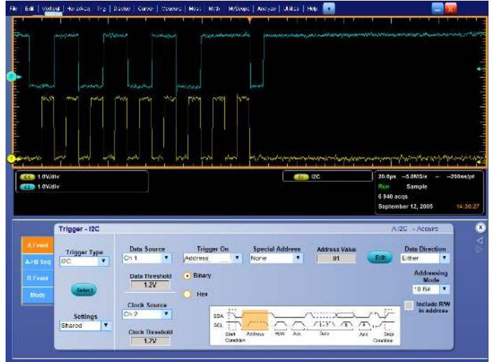
Easily trigger on a specific I2C address.
