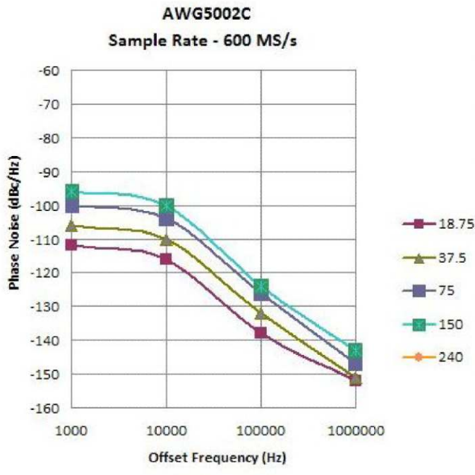
AWG5002C phase noise (typical)
