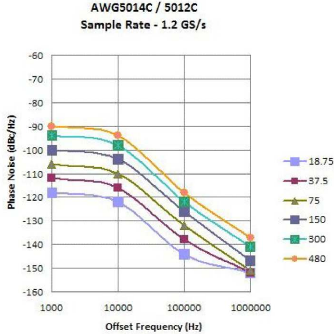
AWG5014C/AWG5012C phase noise (typical)
