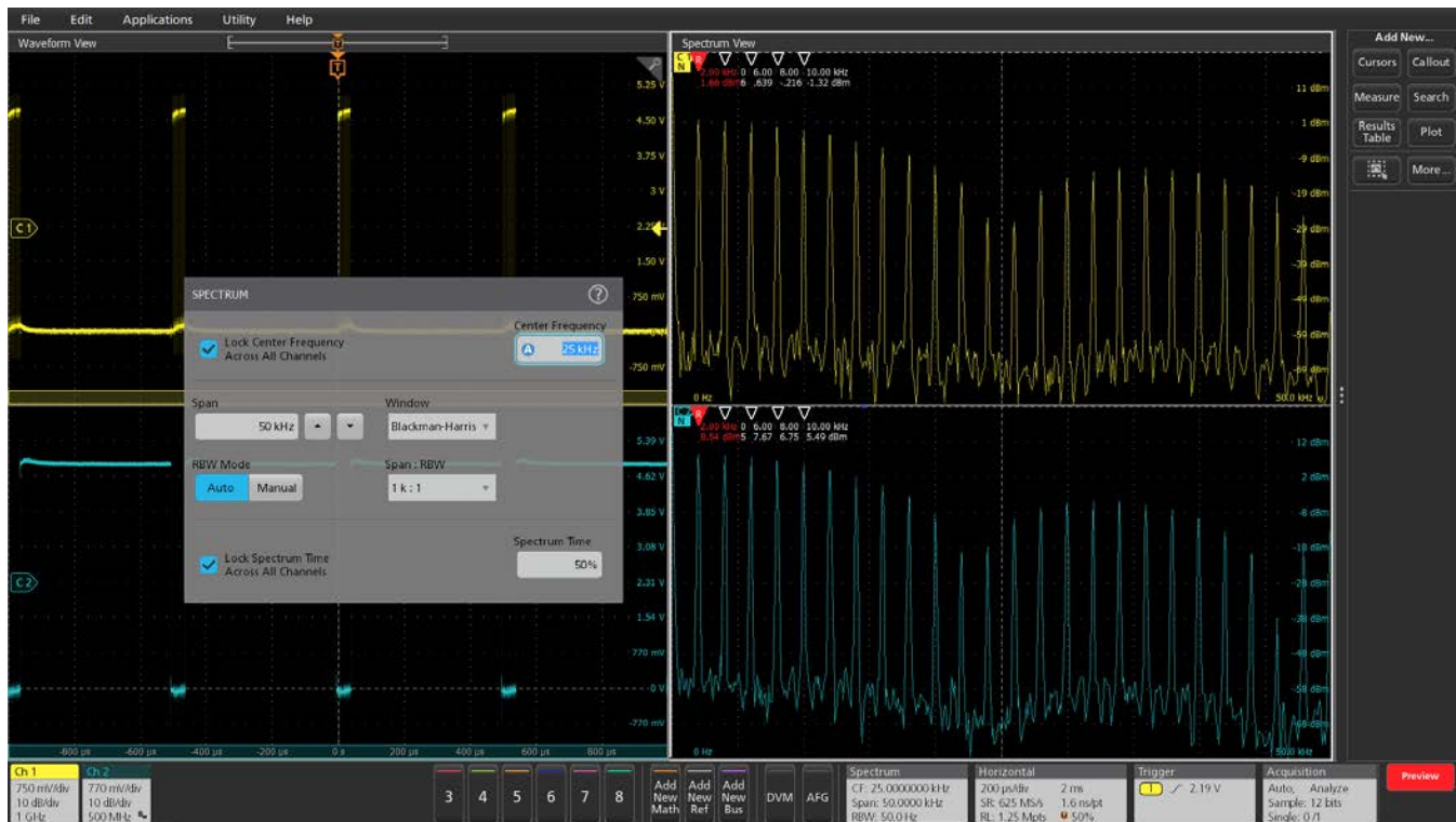
Figure 25: Intuitive spectrum analyzer controls like center frequency, span and resolution bandwidth (RBW), independent from time domain controls, provide easy setup for frequency domain analysis. A spectrum view is available for each FlexChannel analog input, enabling multi-channel mixed domain analysis.
