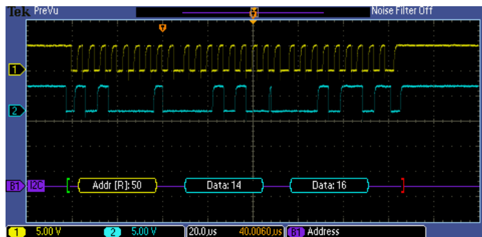
Triggering on a specific data packet going across an I 2 C bus. The yellow waveform is the clock and the blue waveform is data. A bus waveform provides decoded packet content including Start, Address, Read/Write, Data, and Stop.
