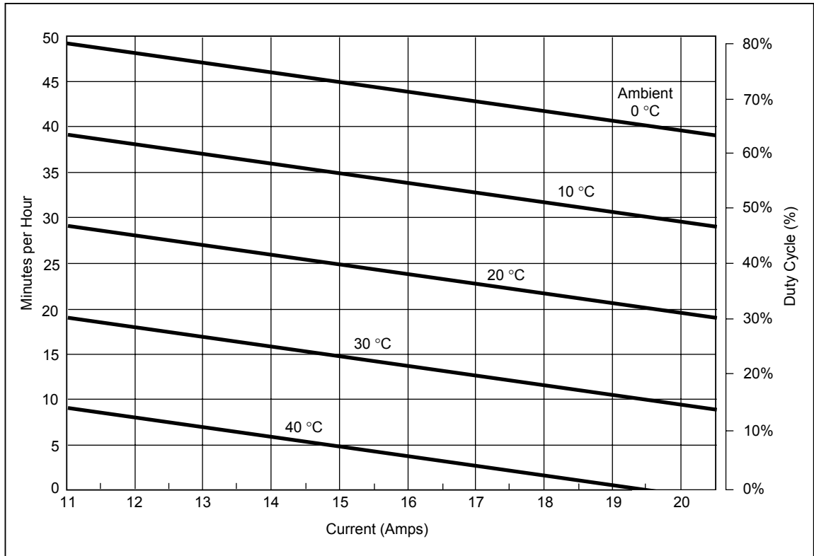
Figure 1. Allowable Duration of Current >11 A
