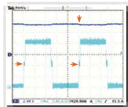
Figure 4 : Parallel non-synchronous dynamic loading
